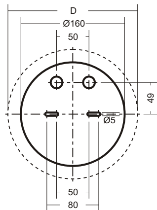
D 200/250
