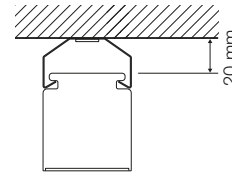
Mounting clamps for ceiling mounting
